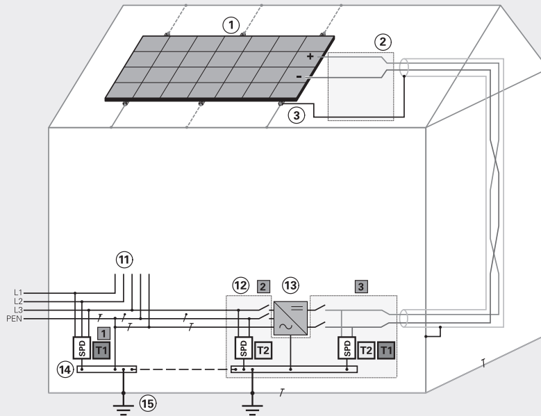
7.12.4 Figure 9: Variante xC
